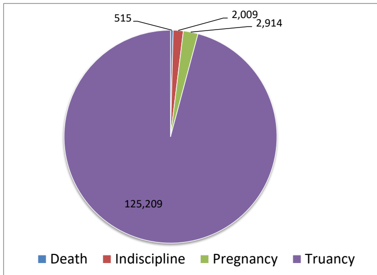
Chart 3.7: Number of Dropouts in Government and Non-Government Schools by Reason, 2021
